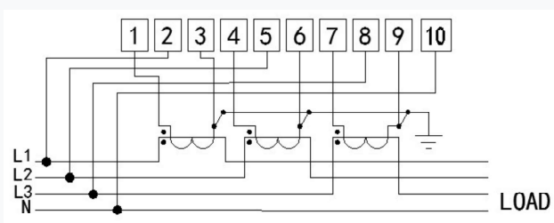
3 Phase 4 Wire Connection
